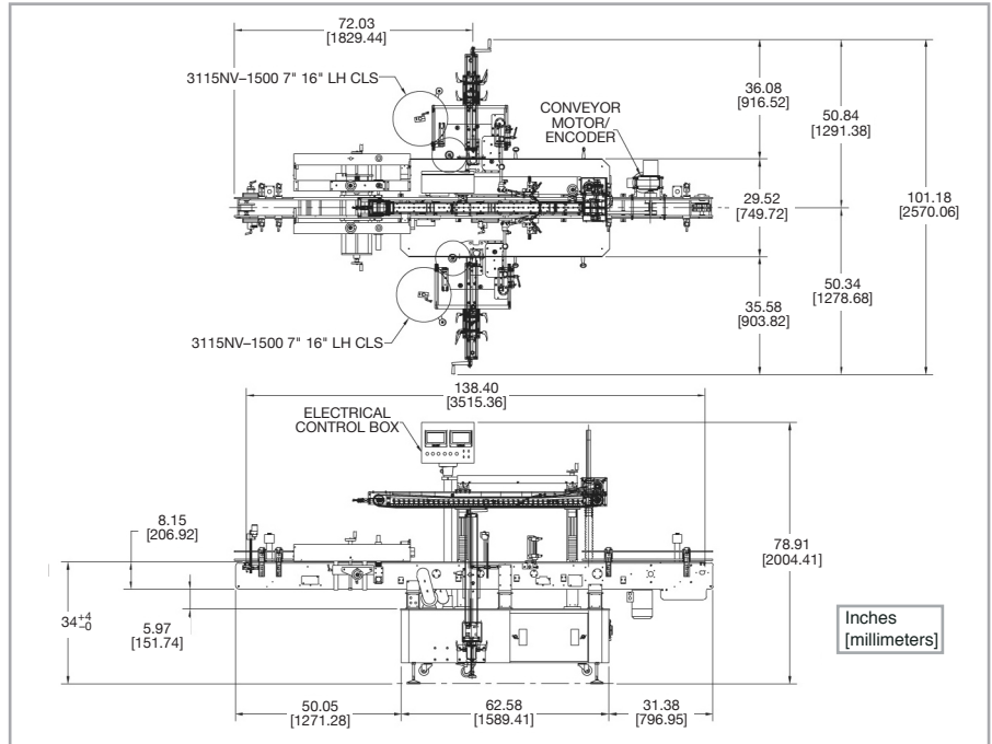
Stated dimensions are approximations. Please consult factory if dimensions are required for line integration.
